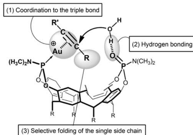
Figure 2. Three strategies of 1 ·Au + in the selective hydration of internal alkynes (the two quinoxaline walls are omitted for ease of viewing): (1) coordination of Au + toward the triple bond, (2) hydrogen bonding between P=O and H 2 O, and (3) the inner space favorably includes one side of the alkyne substituents.
