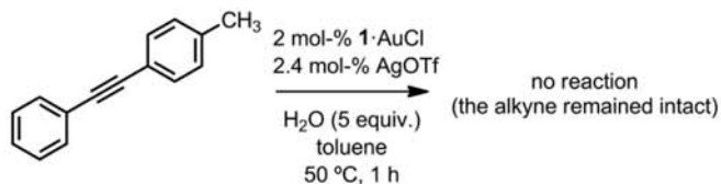
Scheme 2. Reactivity of 1-methyl-4-(phenylethynyl)benzene at 50 °C in the presence of 1 -AuCl.
