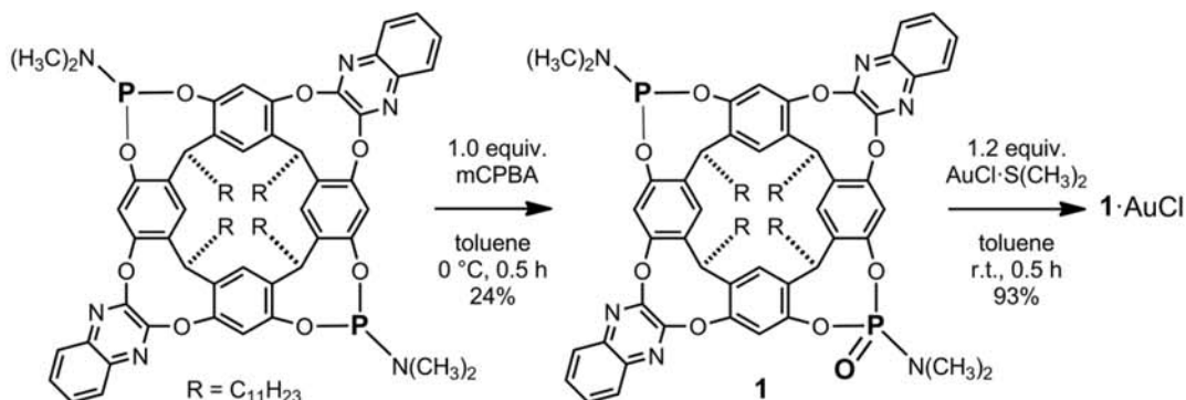
Scheme 1. Synthesis of 1 ·AuCl derived from cavitant 1 prepared by m CPBA oxidation.
