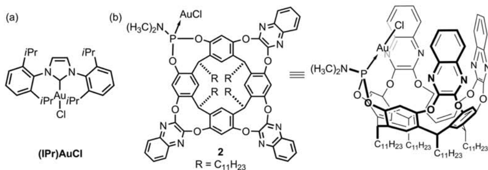
Figure 3. (IPr)AuCl, and mono-AuCl 2 tethered to a triquinoline-spaced resorcin[4]arene. A part of the quinoxaline moiety is colored in gray for ease of viewing.
