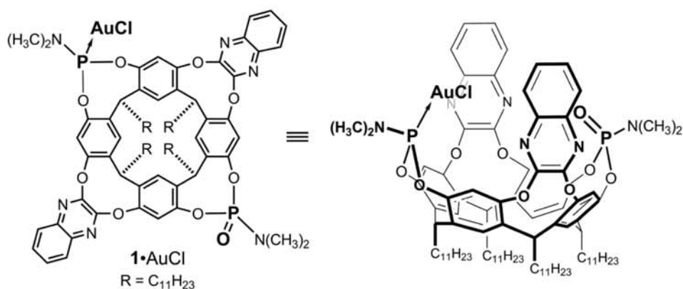
Figure 1. Mono-Au complex cavitand 1·AuCl functionalized with PNMe 2 and O=PNMe 2 moieties in which the two P–N bonds point outside toward the cavity space. A part of the quinoxaline moiety is colored in gray for ease of viewing.
