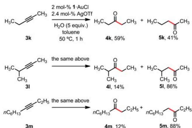
Scheme 3. Ability of 1 -AuCl to catalyze the selective hydration of 2-pentyne ( 3k ), 4-methyl-2-pentyne ( 3l ), and 3-decyne ( 3m ). Yields were determined by 1 H NMR spectroscopy analysis of samples purified by short-plug silica gel column chromatography eluting with [D 8 ]toluene. The 1 H NMR spectra of 4k , 5k , 4l , and 5l were inferred from ChemDraw-estimated charts. The 1 H NMR spectra of 4m and 5m were identical to those of commercially available 4-decanone and 3-decanone, respectively.
